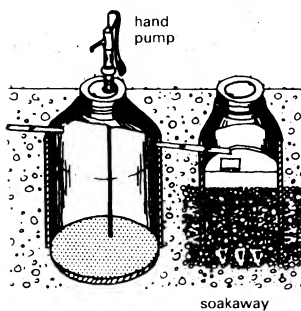
4 Rainwater storage with eco soakaway
